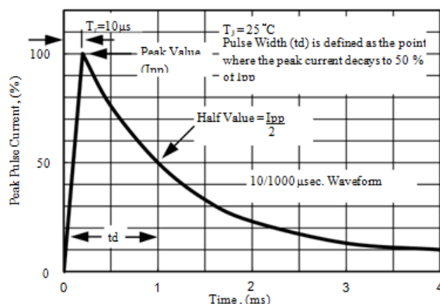
Fig. 2 - Pulse Waveform
